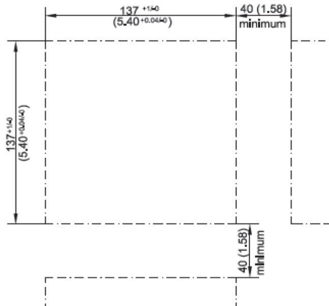
Panel cut-out dimensions
